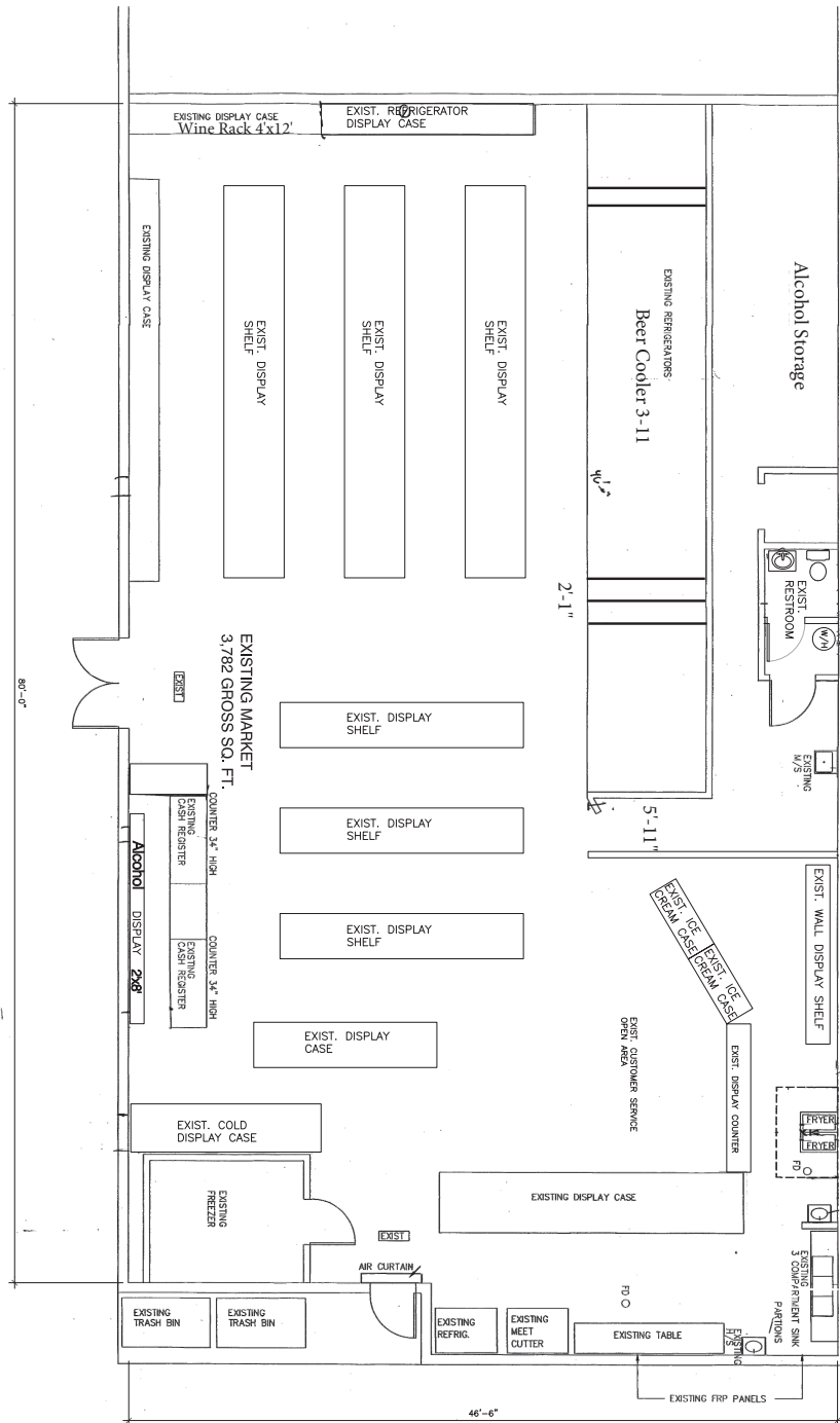
EXISTING MARKET FLOOR PLAN SCALE: 1/4" = 1'-0"
