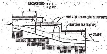
FIGURE 1809.3 STEPPED FOOTING
