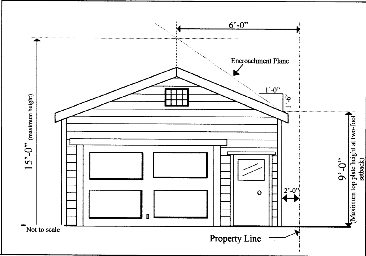
Figure 5-1 Accessory Structure Regulations
