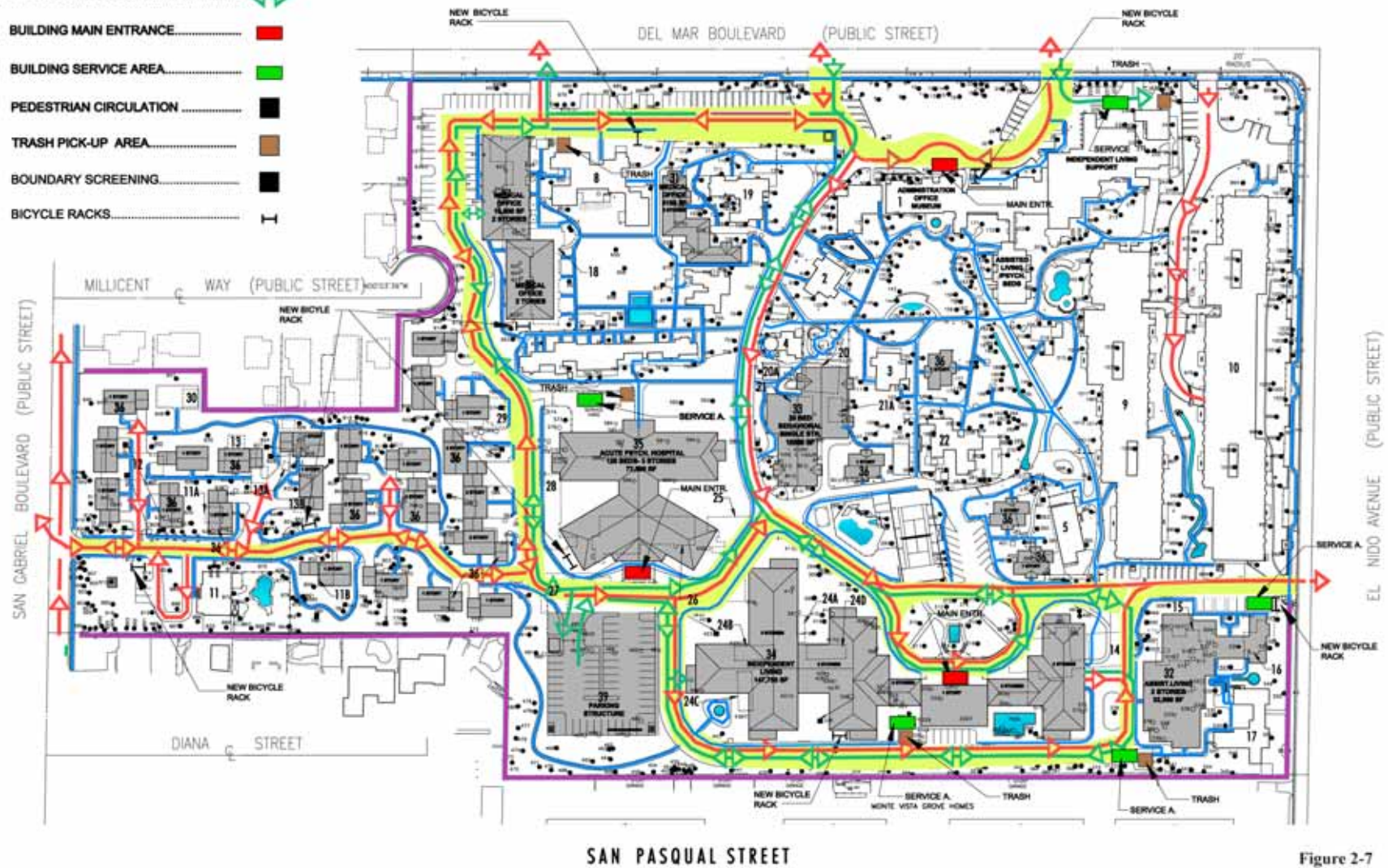
Figure 2-7 Circulation Plan
