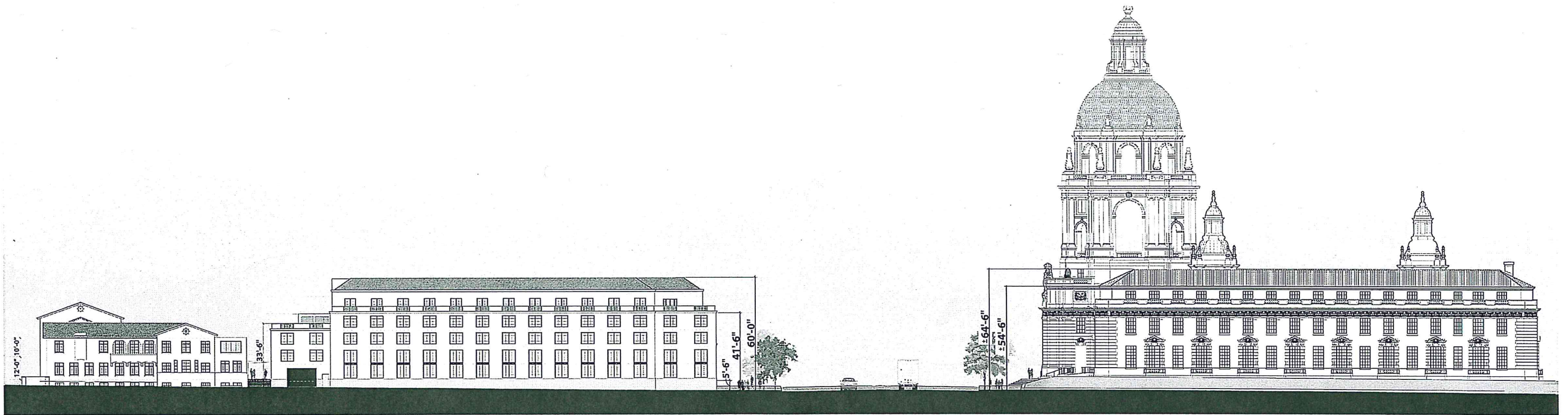
UNION STREET ELEVATION
