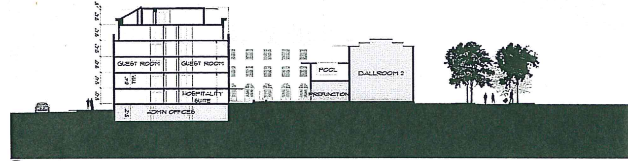
(B) SOUTH-NORTH BUILDING SECTION
