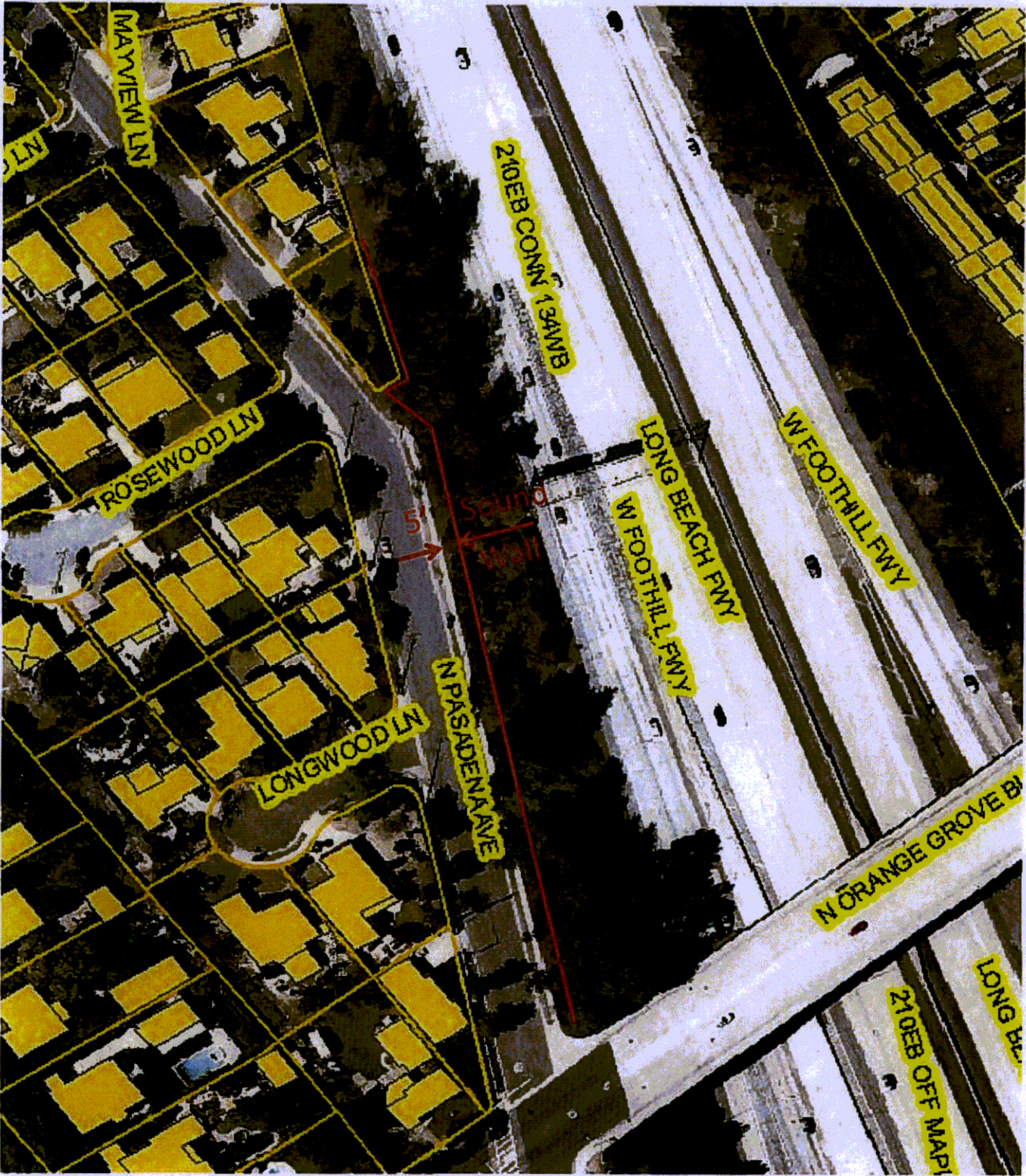
————— 12 FT HIGH SPLIT FACE BLOCK SOUND WALL
